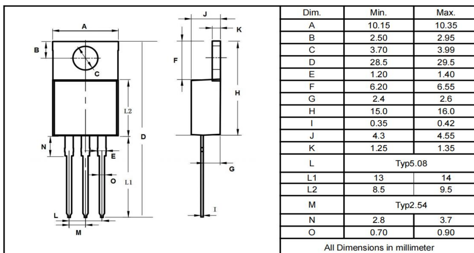
TO-220AB
